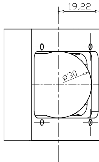
view B
